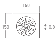
ELS-7116 Antipest Floor Trap Grating
