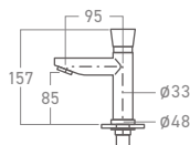
EL-SS76BDA Self-closing Basin Cold Tap
