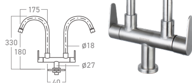
EL-SS9900P Double Pillar Cold Tap
