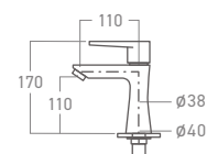
ELS-B7300M Mixer Tap
