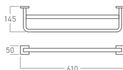
BFC-02DTB Double Towel Bar
