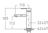
ELS-9988B Basin Cold Tap
