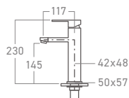
EL-SS6005 Mixer Tap
