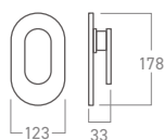
ELS-B8000M Concealed Shower Mixer Solid Brass with Chrome Finish
