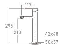
EL-SS6008 Mixer Tap
