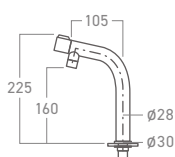
EL-SS33B Basin Cold Tap
