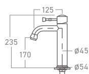
ELS-388FBM Mixer Tap (Brass)
