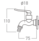
ELS-886W Wall-Mounted Cold Tap
