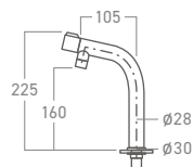
EL-SS33B Basin Cold Tap
