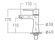
ELS-B7300M Mixer Tap
