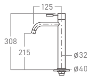
ELS-9800B Basin Cold Tap
