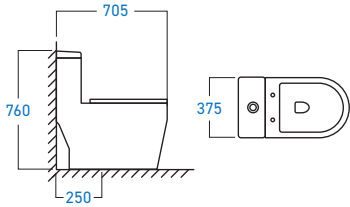
WC-1832WD ONE-PIECE WASHDOWN DUAL FLUSH S-TRAP / P-TRAP ROUGHING-IN
