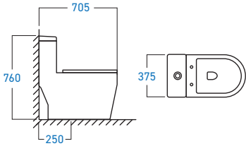
WC-1832WD ONE-PIECE WASHDOWN DUAL FLUSH S-TRAP / P-TRAP ROUGHING-IN
