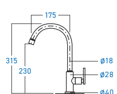
ELS-9011P PILLAR COLD TAP
