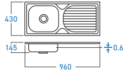
ELS-1320S DRAIN BOARD KITCHEN SINK
